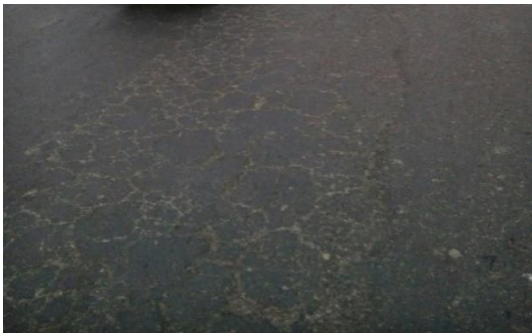
Figure 3 Alligator cracking at Chaprashhi Pura
