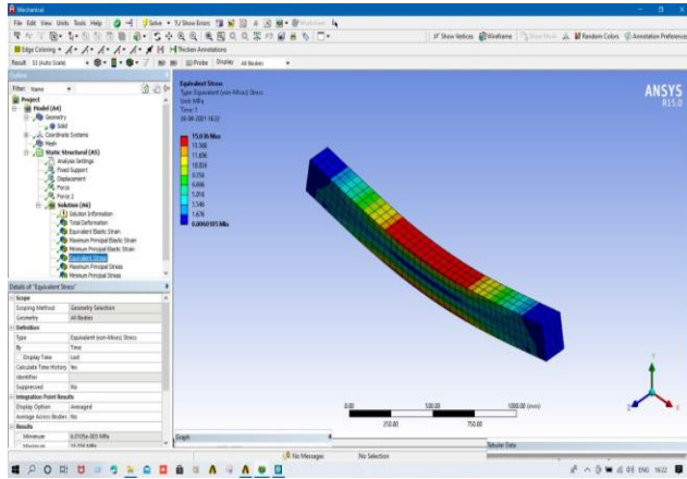
FIG 16. Equivalent Stress
