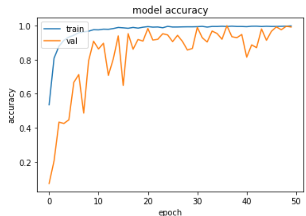
Chart -2: Model Accuracy Chart
