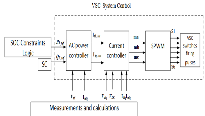
Figure 4: Schematic diagram of the control system of the BESS.
