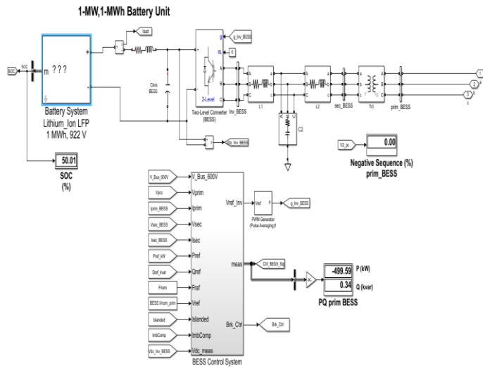
Figure 8 Battery back Unit
