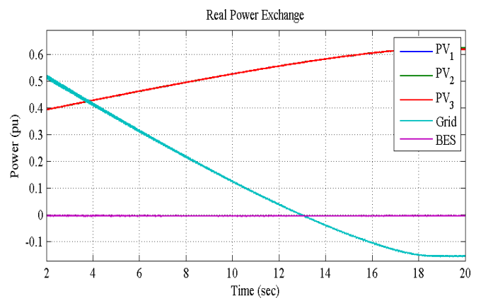
Figure 5 (a) Real power exchange between the three Solar-PV systems, the utility grid, and the BESS when the battery is idle (pu)
