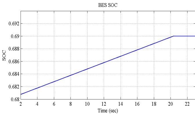
Figure 5 (b) Battery SOC is within the pre-specified range (0.73)
