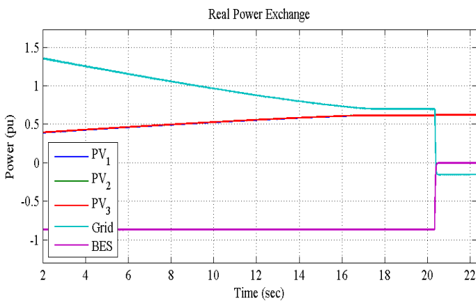
Figure 6 (a) Real power of the three Solar-PV systems, the utility grid, and the BESS when the battery is under the charging mode (pu)
