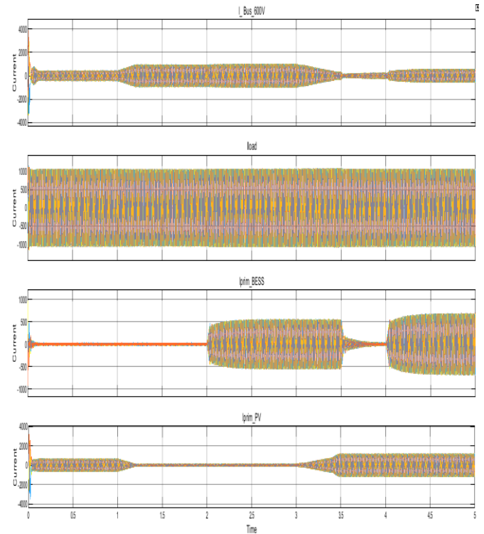
Figure 11 Current Variation of system Solar, grid, BESS to maintain load current.
