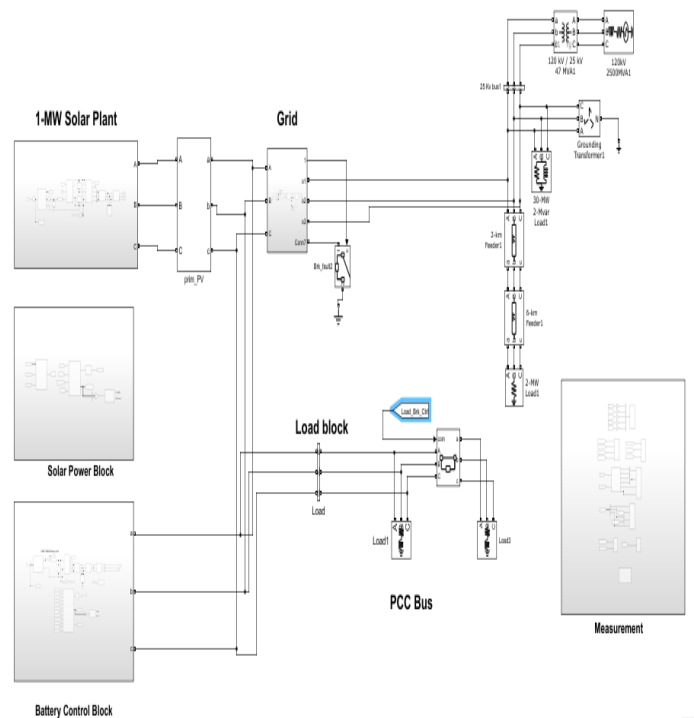
Figure 7: Simulink model of microgrid
