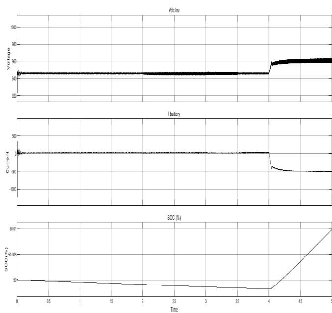
Figure 9 Voltage, current and SOC of the battery.
