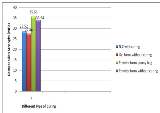
Fig 3.3: Compression Strength for powder Form Curing.
