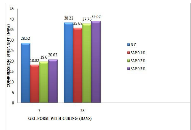
Fig 3.1-Compression Strength for Gel Form Pond Curing.
