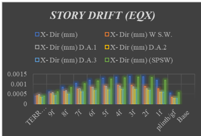
Figure 4.7 STORY DRIFT
