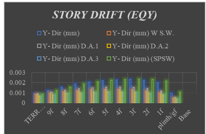
Figure 4.8 STORY DRIFT
