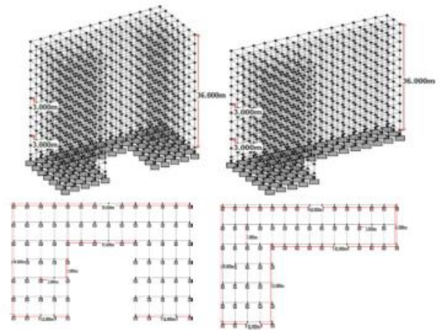
Fig 2 & 3. 3D ELEVATION AND PLAN OF C & L SHAPE OF BUILDING
