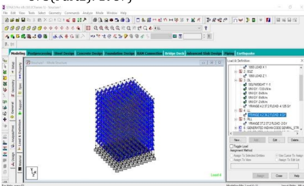
Fig 9. LIVE LOAD IN X AND Z DIRECTION
