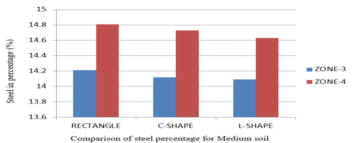
Chart 8. Comparison of steel percentage (%) for Medium soil
