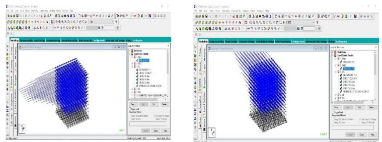
Fig 4 & 5. EARTHQUAKE LOAD IN X AND Z DIRECTION
