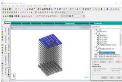
Fig 10.ROOF LIVE LOAD IN X AND Z DIRECTION
