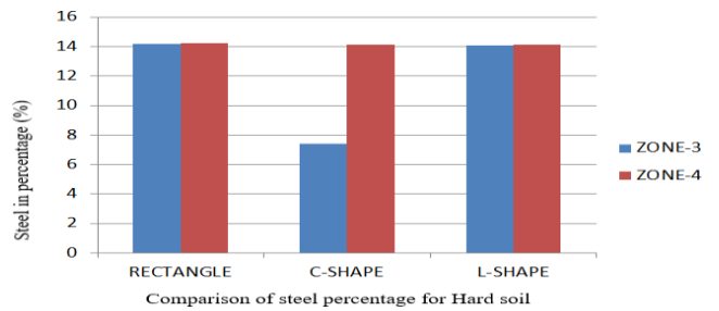
Chart 7. Comparison of steel percentage (%) for Hard soil
