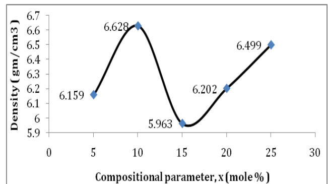
Fig-5: Variation of Density with compositional parameter of xZnO-(30-x)Na_2O-36Bi_2O_3-34B_2O_3 glass system
