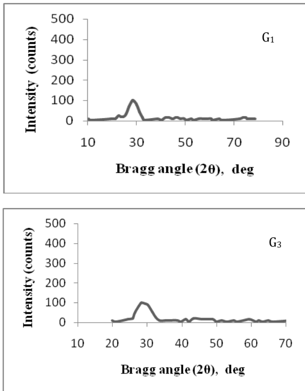
Fig-2: X-ray diffractograms of the glass G 1 and G 3
