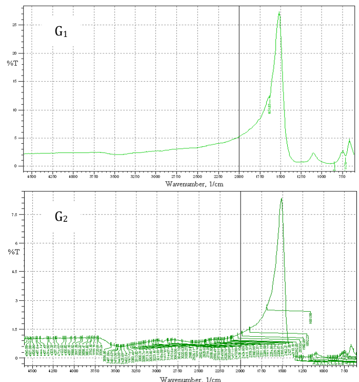
Fig-3: FTIR transmission spectra of glasses G 1 and G 2
