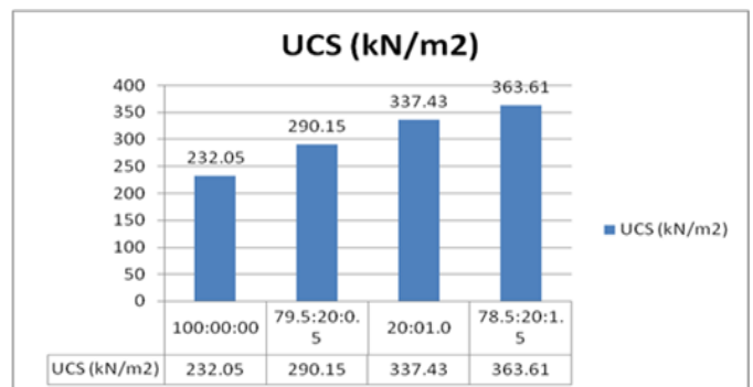
Chart-2: Variations b/w UCS Values of Clayey soil, Sugercane Bagasse Ash and Nylon Fibre with different proportions
