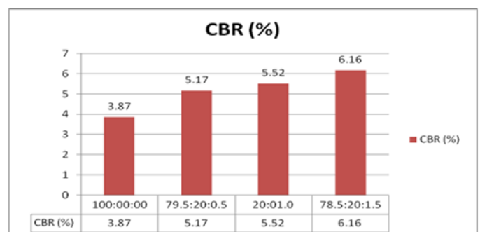
Chart-3: Variations b/w CBR Values of Clayey soil, Sugercane Bagasse Ash and Nylon Fibre with different proportions
