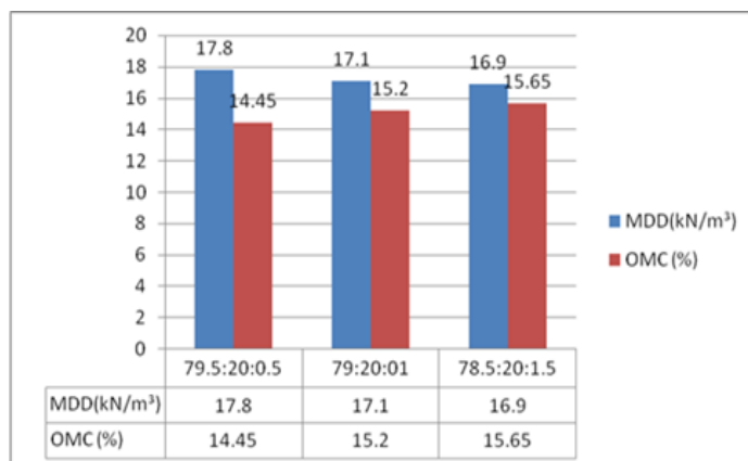
Chart-1: variations b/w MDD and OMC of SCBA, Nylon Fibre & soil with different proportions
