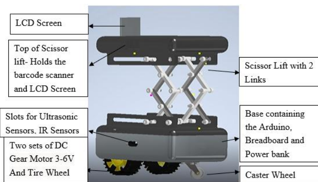
Fig -2: CAD Model Rendering
