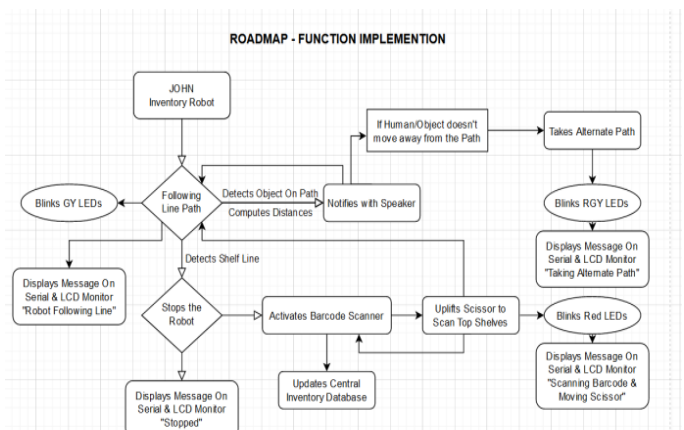
Fig 10: Algorithm Implementation Roadmap
