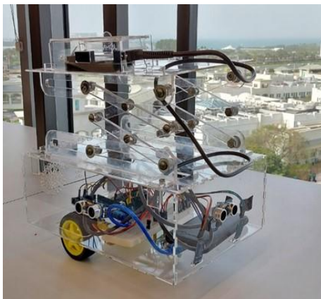
Fig 12: Final look of the robot"
