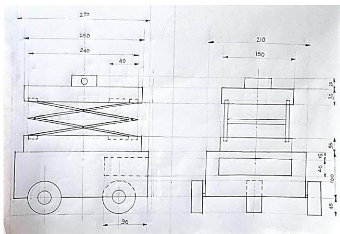
Fig -1: Mechanical Design
