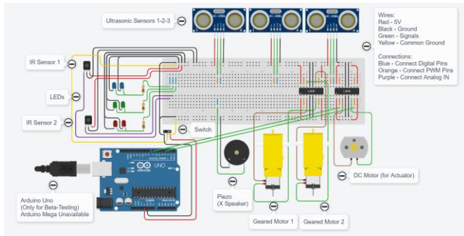
Fig 11: Design and Wiring Simulation of Robot
