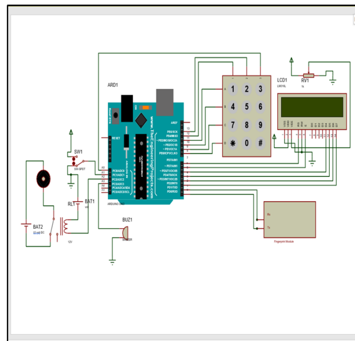
Fig 3. Circuit Diagram
