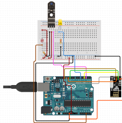
Fig -3: Circuit Diagram of Transmitter Section
