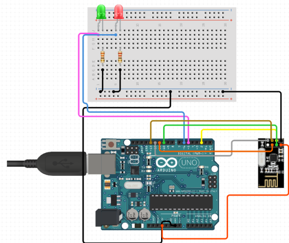
Fig -4: Circuit Diagram of Receiver Section
