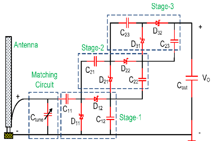
Fig 3 3 Stage Voltage multiplier Circuit
