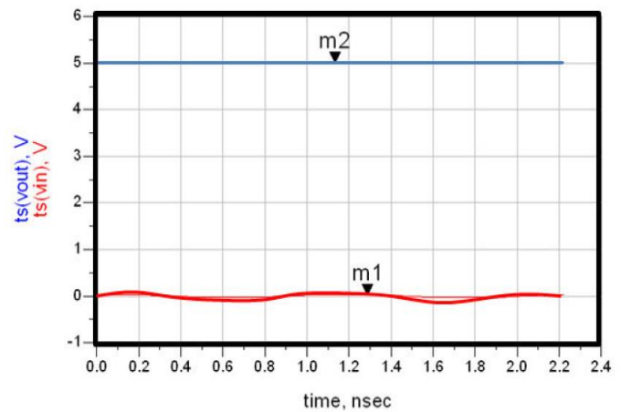
Fig. 4.5 simulation result 3 stage voltage multiplier with matching circuit
