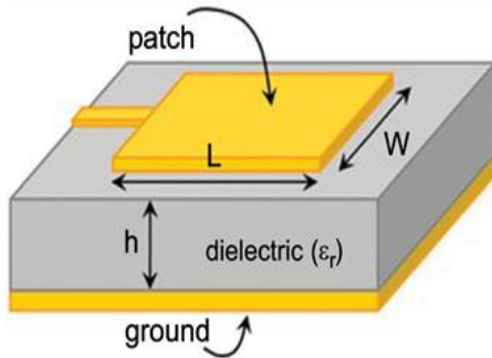
Fig. 2 Microstrip patch antenna
