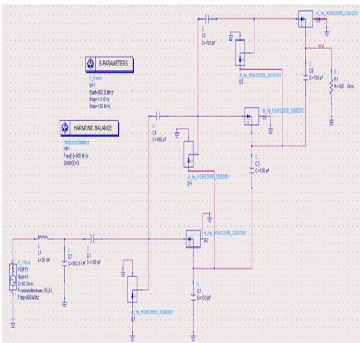
Fig.4.3 Design of 3 stage voltage multiplier using ADS software
