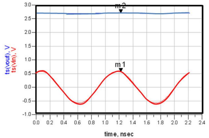
Fig. 4.4 simulation result of 3 stage voltage multiplier using ADS software
