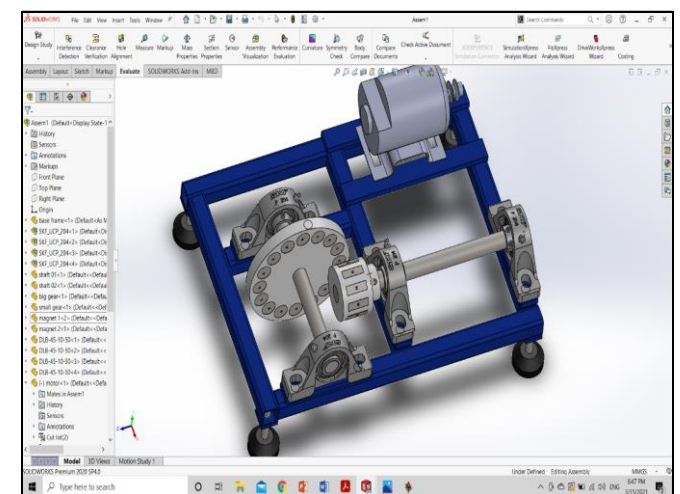
Fig 11: Assembly of prototype model
