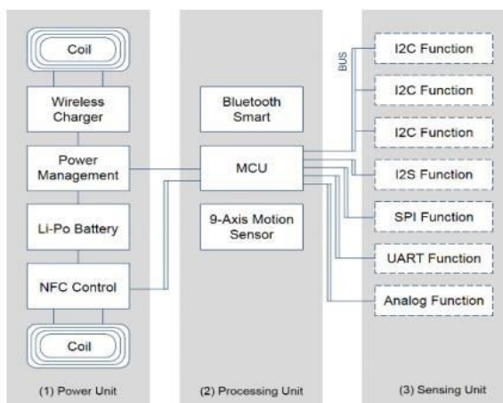
Fig -3: MorSensor Architecture, Power Unit, Processing Unit, Sensing Unit[6]
