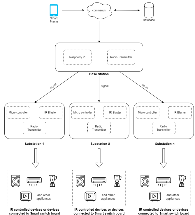
Fig -6: Architecture
