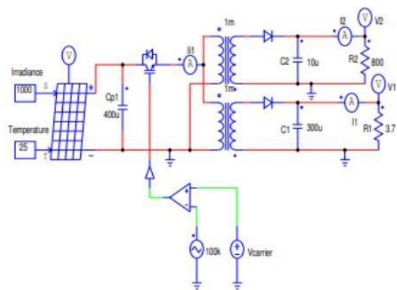
Fig -2: Circuit diagram of energy harvesting system with fly-back converter
