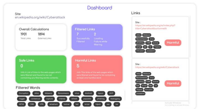
Fig.5:- Harmful word displayed
