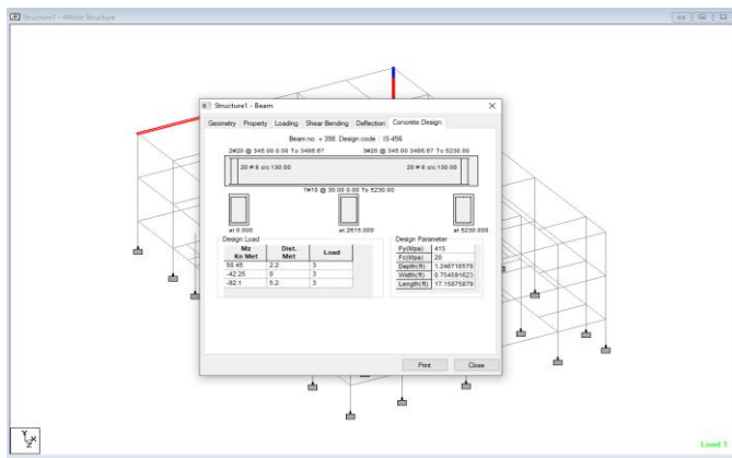
Fig -11: Detail Design of Beam
