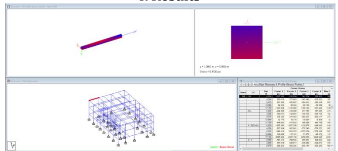
Fig -9: Beam Stress Contour
