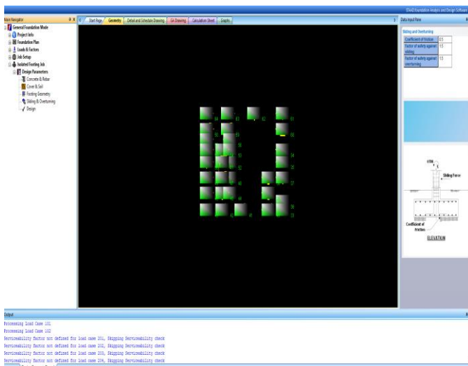
Fig -13: Detail Design of Footing
