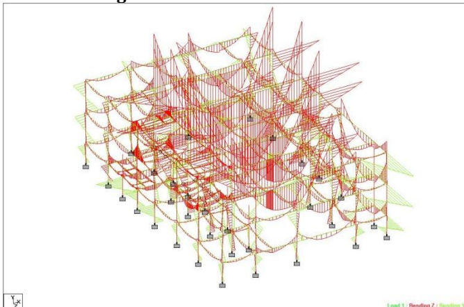
Fig -7: Bending Moment in Z and Y Direction
