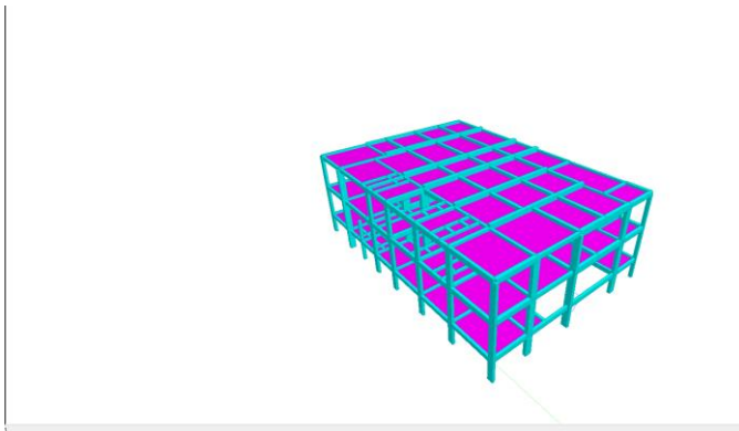
Fig -4: 3D rendering View of Model
