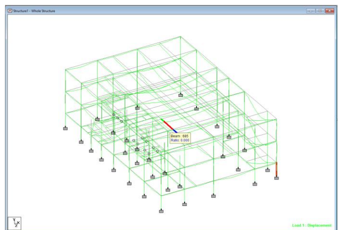
Fig -10: Deflection in Structure
