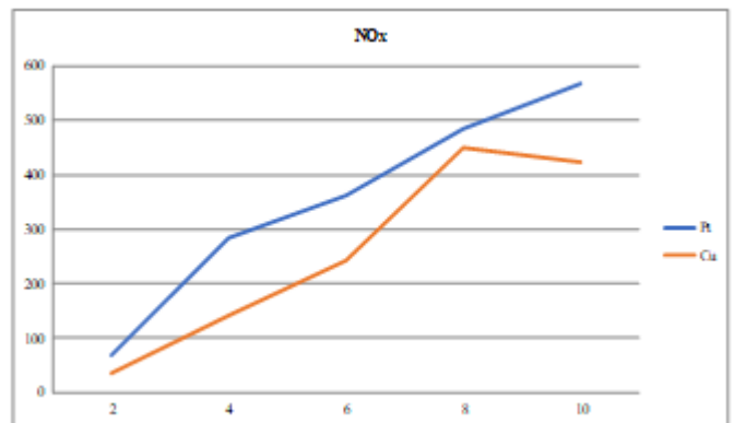
Chart -9: Cu & Pt NO x graph
