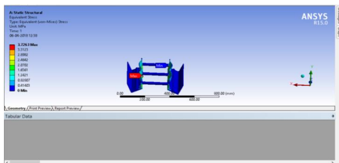
Fig.3 Von-Mises Stress Analysis
