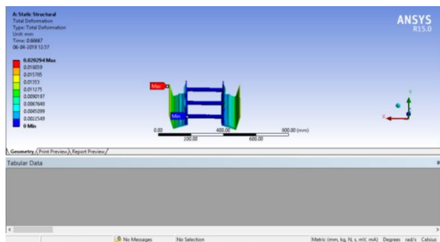
Fig.2 Total Deformation
