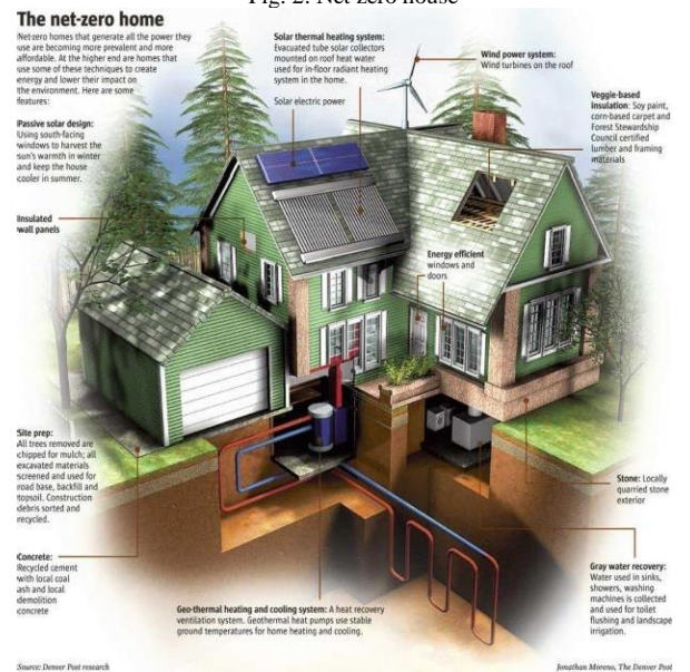
Fig. 2: Net zero house
