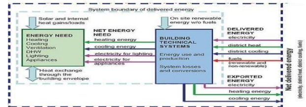
Fig. 6 : Net delivered energy
