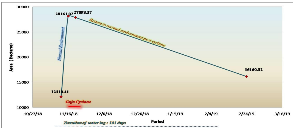
Fig-5: Waterlog areas pre and post 'Gaja' cyclone in southern Nagapattinam district
