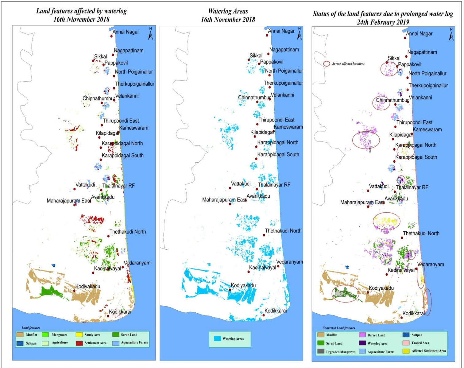
Fig-10: Significant impact of prolonged waterlog on land features
