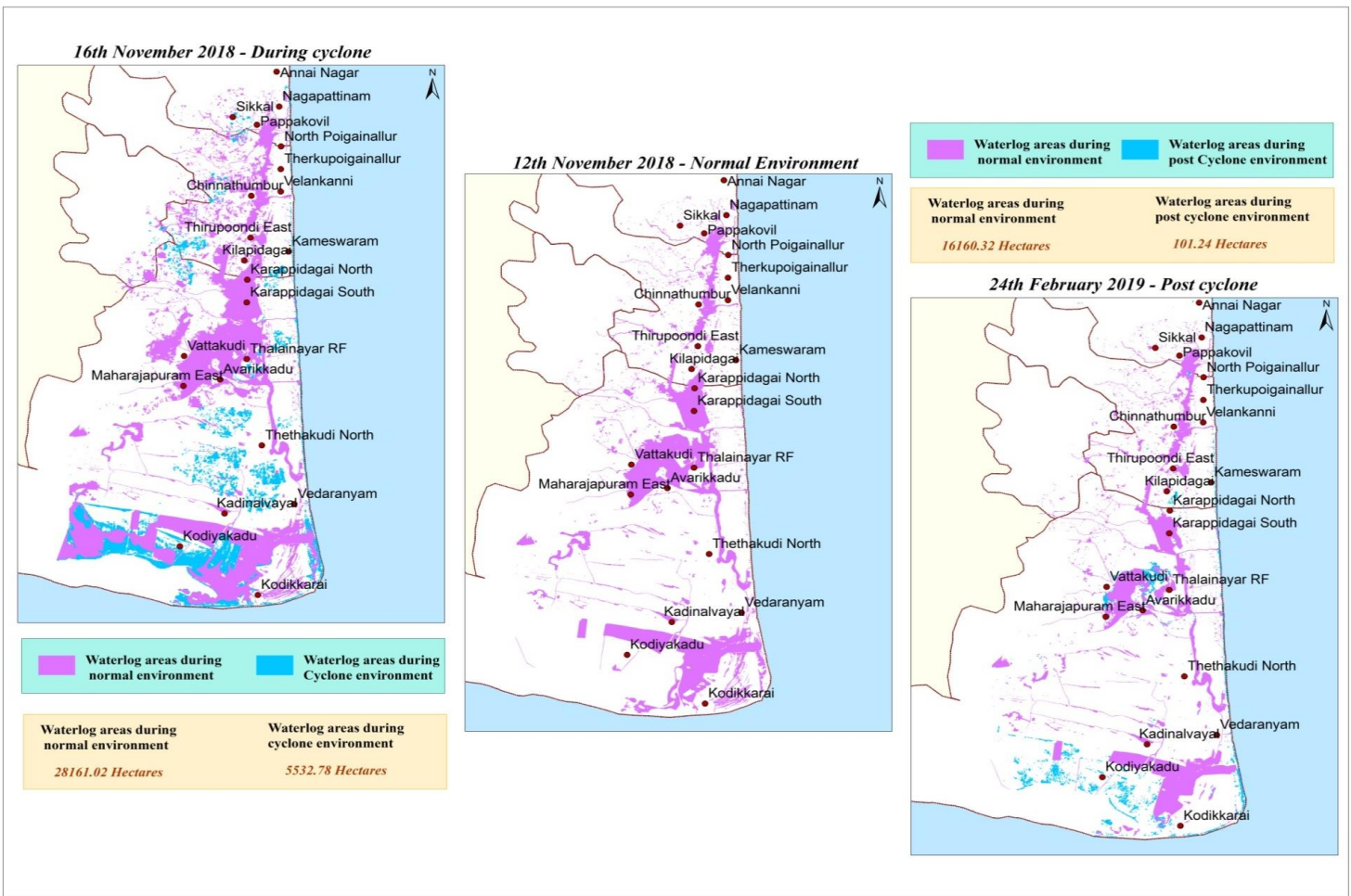
Fig-9: Water log areas during hazard and non-hazard conditions of South Nagapattinam
