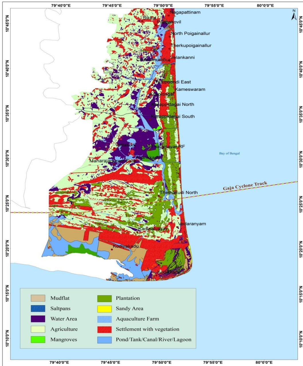
Fig-8: Land features in the study area (20 th November 2018)
