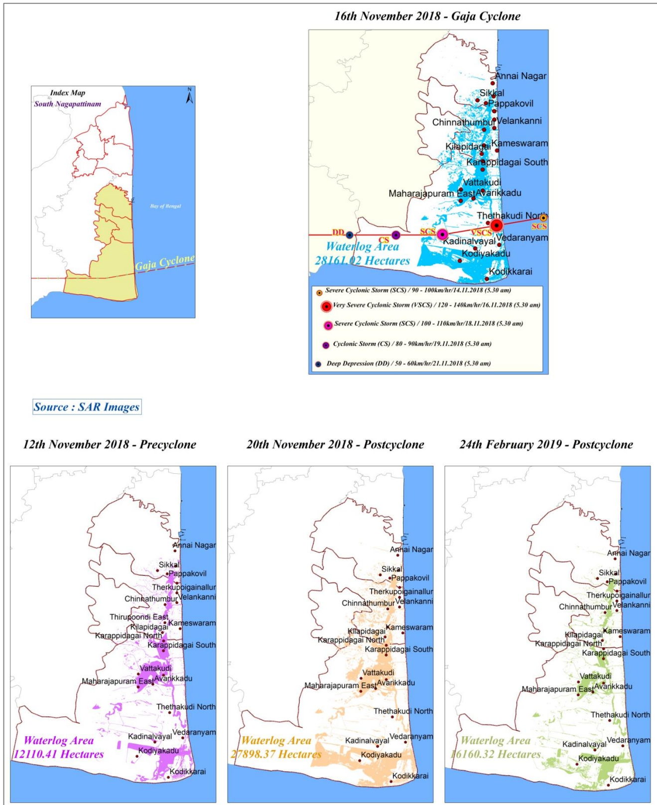
Fig-7: Temporal waterlog areas pre and post Gaja cyclone in southern Nagapattinam district
