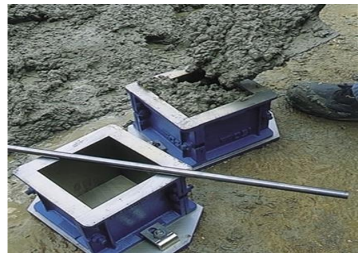
Fig 7. Mould preparation
