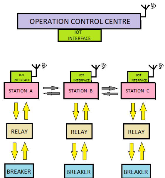
FIG 1 - Block Diagram IOT Based Substations.
