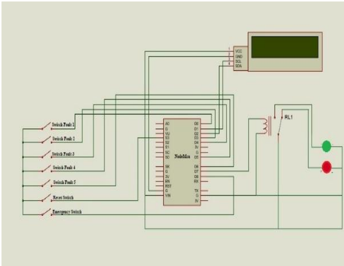
FIG 2- Demo Model of The IOT Based Substation.
