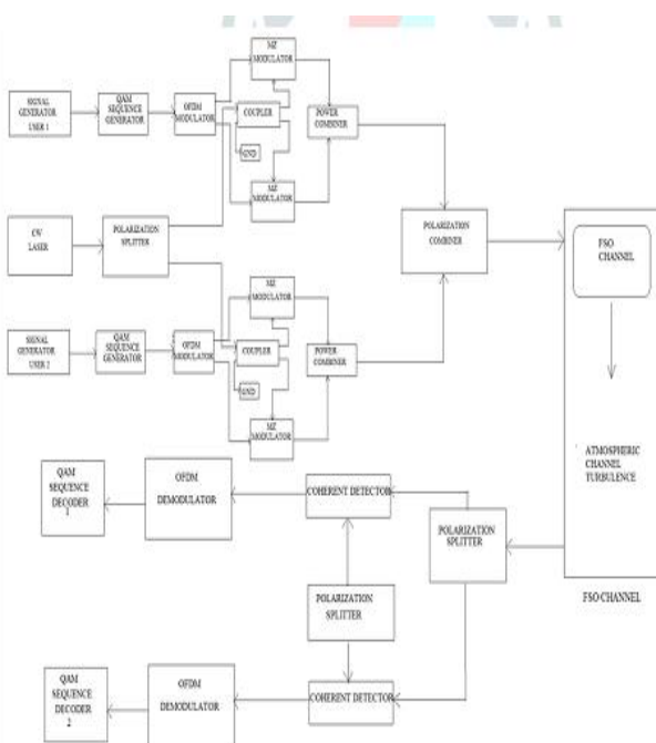
Figure 1. Block diagram of PDM-OFDM FSO system
