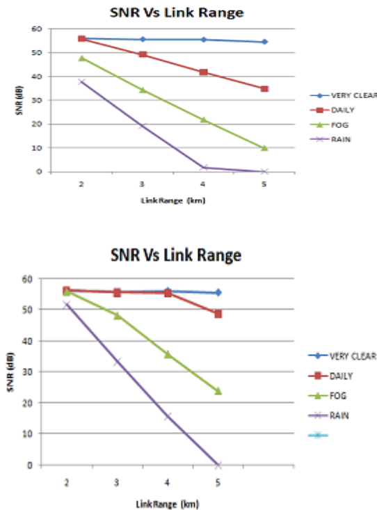
Figure 8 SNR Vs Link Range for OFDM and PDM-OFDM FSO system.
