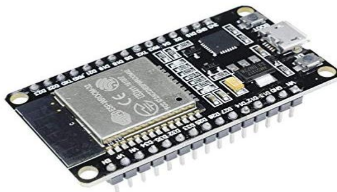
Fig.5 ESP 32 Micro-Controller
