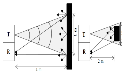
Fig. 9 Ultrasonic Sensor Detecting Obstacles
