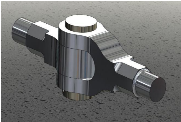
Fig 3.4 MECHANICAL JOINT
