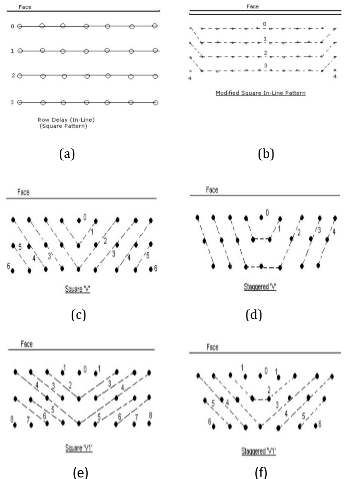
Fig-3 Sequence of initiation in multi-row blasting
