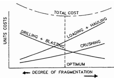
Fig-4 Optimum fragmentation
