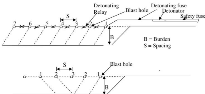
Fig-2 Sequence of initiation in single row blasting
