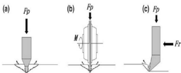
Fig-1 Types of rock breakage during drilling: (a) percussive, (b) rotation, (c) cut.
