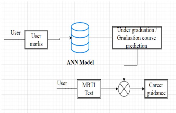
Fig -1: ANN Model of proposed system
