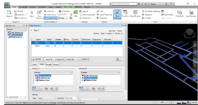
Fig.11: Clash detective test with zero clash
