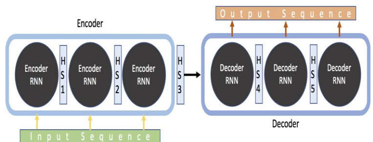
Figure 3: Seq2seq Model
