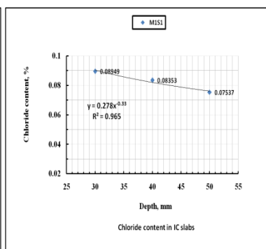
Fig.2b Cl - in impregnation concrete slabs
