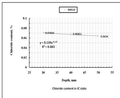
Fig.3d Cl - in impregnation concrete slabs
