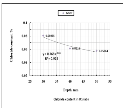
Fig.3a Cl - in impregnation concrete slabs
