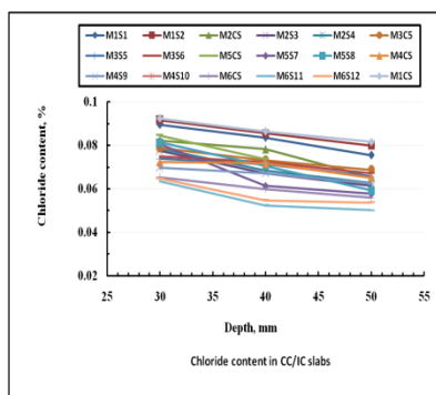
Fig.2a Cl - in CC/IC concrete slabs
