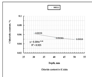
Fig.3e Cl - in impregnation concrete slabs
