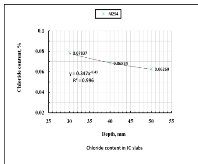
Fig.2d Cl - in impregnation concrete slabs
