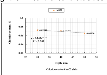
Fig.1d Cl - in control concrete slabs
