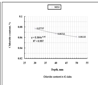
Fig.2e Cl - in impregnation concrete slabs
