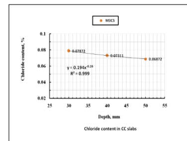
Fig.1c Cl - in control concrete slabs
