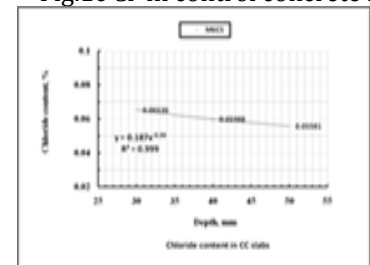
Fig.1f Cl - in control concrete slabs
