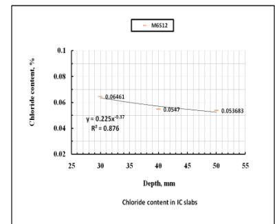
Fig.3f Cl - in impregnation concrete slabs
