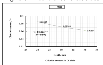
Fig.1e Cl - in control concrete slabs
