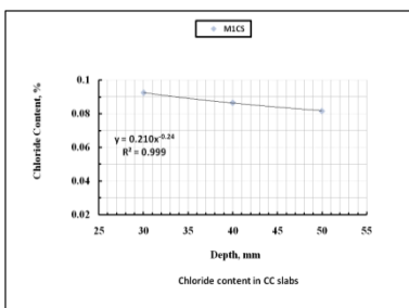
Fig.1a Cl - in control concrete slabs
