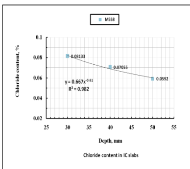
Fig.3b Cl - in impregnation concrete slabs
