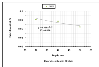
Fig.1b Cl - in control concrete slabs
