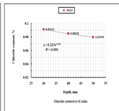
Fig.2c Cl - in impregnation concrete slabs
