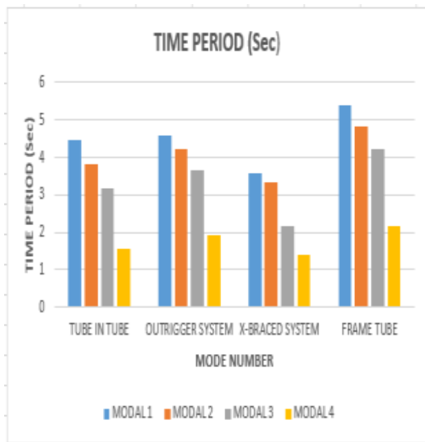
Chart -5: Time Period
