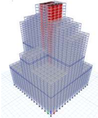
Fig -4: 3D View of Frame Structure with Outrigger System
