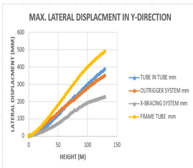
Chart -2: Max. Lateral Displacement in Y-Direction
