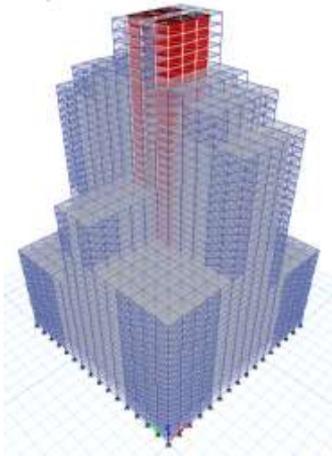
Fig -5: 3D View of Braced Frame Structure
