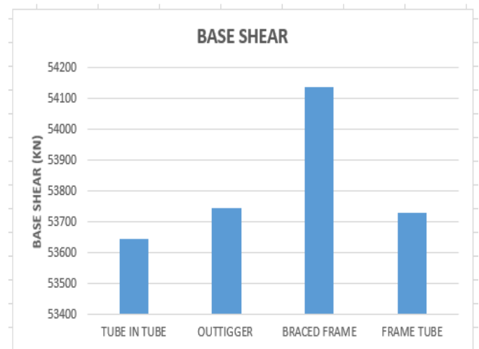
Chart -3: Base Shear
