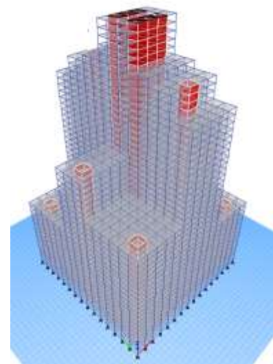
Fig -3: 3D View of Tube in Tube Structure
