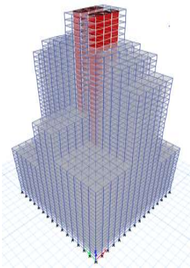
Fig -6: 3D View of Frame Structure
