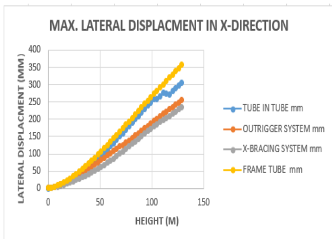
Chart -1: Max. Lateral Displacement in X-Direction
