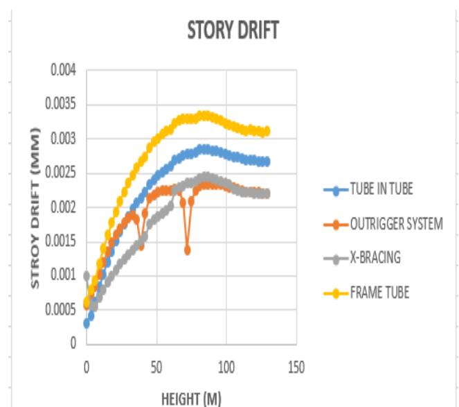
Chart -4: Story Drift
