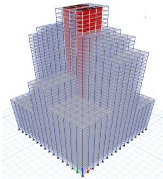
Fig -2: 3D View of model
