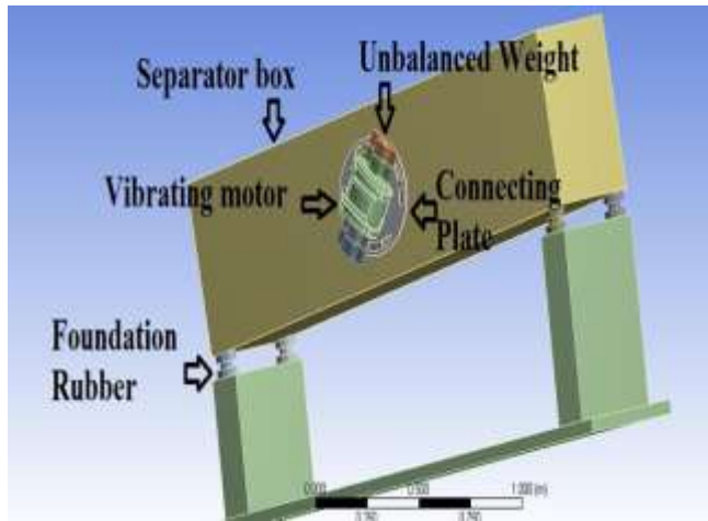
Fig 2: Reciprocating vibro separator assembly
