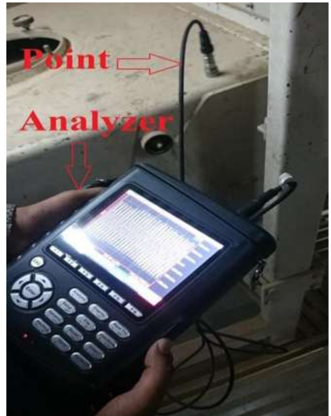
Fig 1: Vibro Analyser
