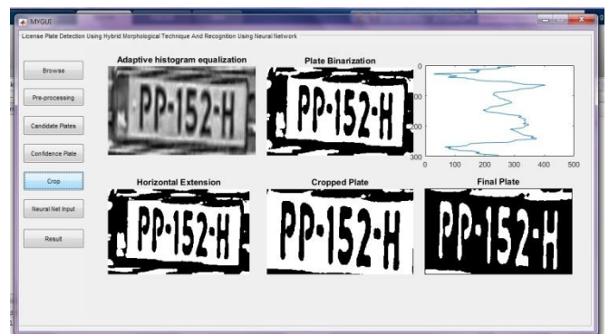
Fig -10: Morphological Processing
