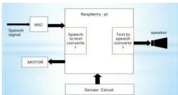
Fig1. Block diagram of chatbot
