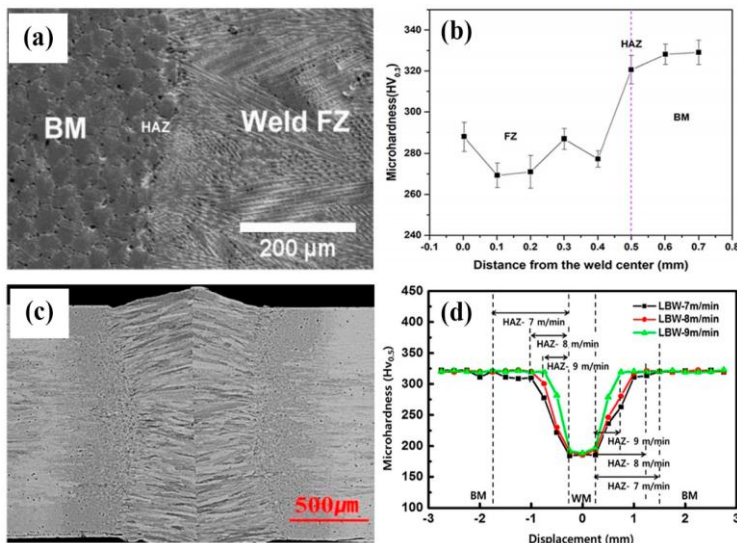
Figure 5. Structure and hardness of laser beam welded Al 0.5 CoCrFeNi HEAs: (a) Welding zones and boundary [30], (b) Microhardness profile on the surface [30], (c) Structure of the welded joints [27] and (d) Hardness distributions in the transverse weld for various welding velocities [27].
