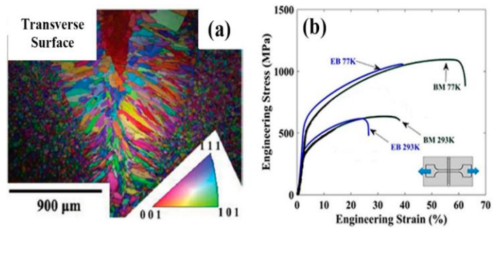
Figure 6. Structures and properties of electron beam butt-welded joints of CrMnFeCoNi alloy:
