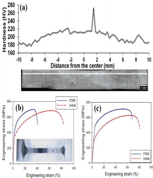
Figure 10. Microhardness distribution across the weld seam (a) and tensile stress-strain curves of the FSW specimens cut across (b) or along (c) the weld seam
