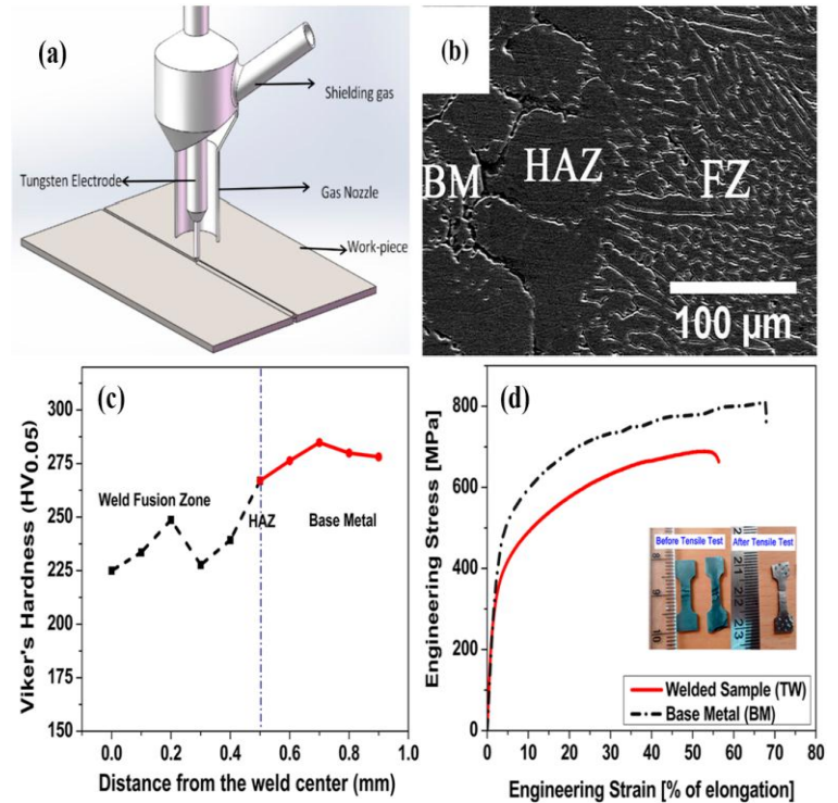
Figure 2. Structure and hardness of the welded zones and engineering stress-stain curves of the welded samples of Al 0.5 CoCrFeNi high entropy alloy (HEA) [19]: (a) Schematic of gas tungsten arc (GTA) welding process, (b) Scanning electron micrographs of base metal (BM)-heat affected zone (HAZ)-fusion zone (FZ) interfaces, (c) Microhardness profile on the surface of the welded sample and (d) Engineering stress-engineering strain curve for the BM and welded sample.
