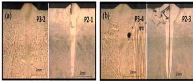
Figure 7. Structures of electron beam deep penetration welding of AlCrFeCoNi HEAs with different heat input: (a) 72 J/mm [32] and (b) 108 J/mm [32].
