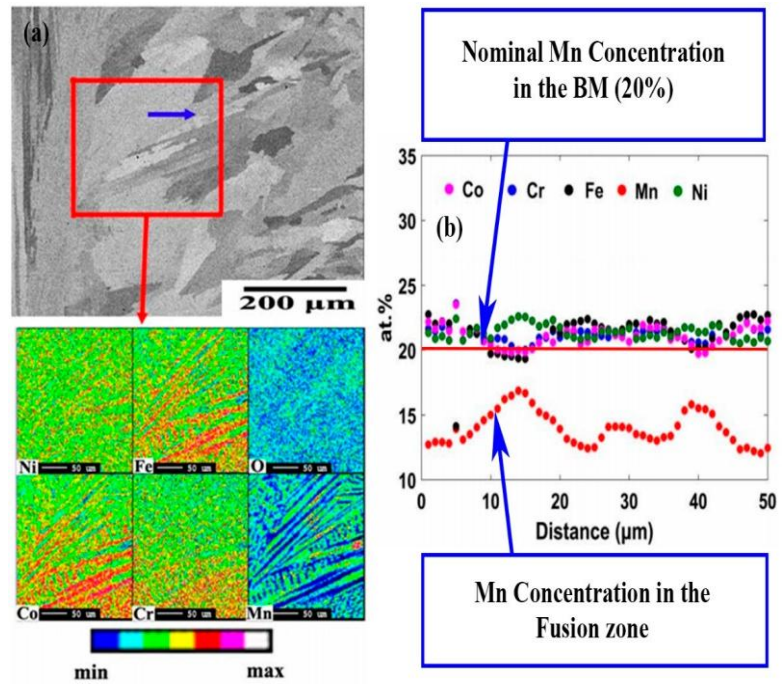
Figure 11. Elemental mapping of fusion zone (FZ) for electron beam welding of CoCrFeMnNi:
