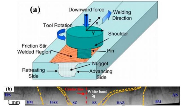
Figure 8. (a) Schematic diagram showing the friction stir welding (FSW) process and (b) Microstructure formed in FSW of Co16Fe28Ni28Cr28 alloys [34]: stir zone (SZ), thermomechanically affected zone (TMAZ), heat affected zone (HAZ) and BM.
