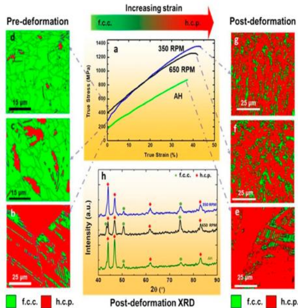
Figure 12. Structure and stress strain curves of high entropy alloys (HEAs) with enhanced properties through friction stir welding.
