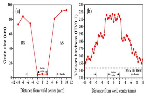
Figure 9. (a) Grain size at different distance from weld center positions and (b) Vickers hardness in the cross-section of FSW CrMnFeCoNi HEA
