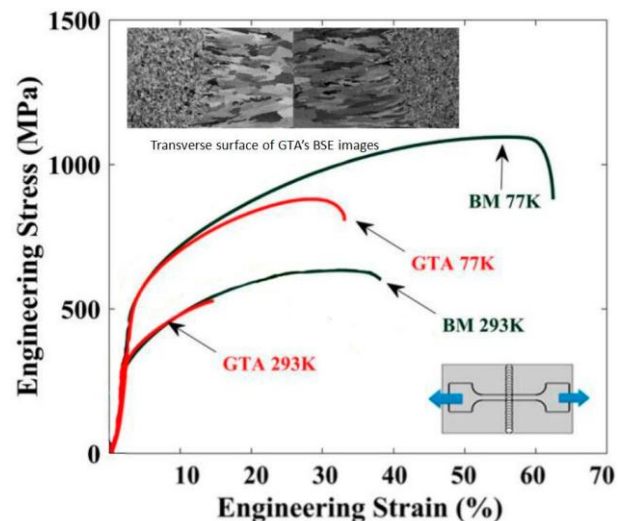
Figure 3. Structure of the welding zones and tensile test results of welded joint of CoCrFeMnNi alloy by GTA [20].
