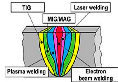
Figure 1. Welded zones formed by different welding methods. [ http://is.gliwice.pl/en/strona-cms/electron-beam-welding-laboratory ].
