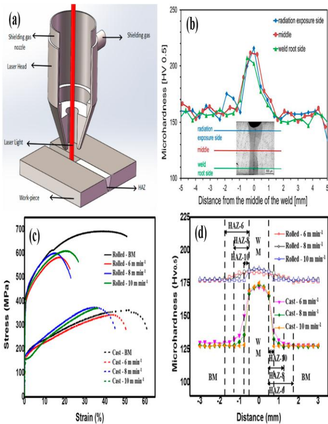
Figure 4. Hardness distribution in laser welded joints of HEAs: (a) Schematic diagram showing the laser welding process, (b) Microhardness profile of a butt-joint [26], (c) Stress-strain curves of the cast and rolled BM at various welding velocities [28] and (d) Hardness distribution in the transverse welds of the cast and rolled HEAs at various welding velocities: 6–10 m min -1 [28].
