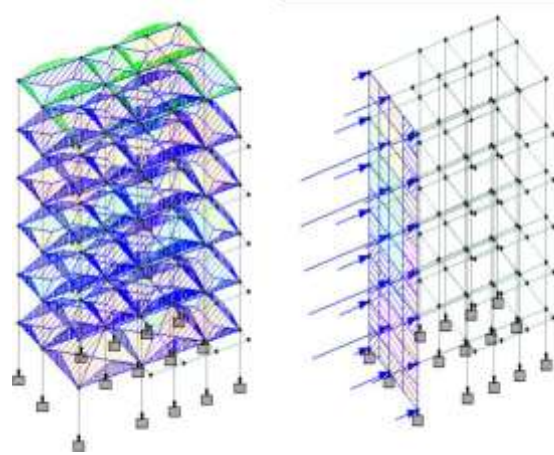
Fig.2 Diagram of Live load & wind loads
