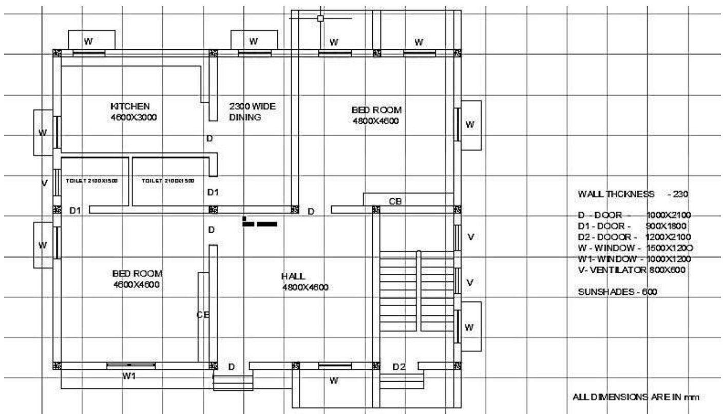
Fig.1 Plan of the multistory building
