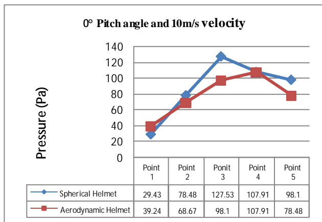
Graph7. At 0°Pitch angle and 10m/s velocity
