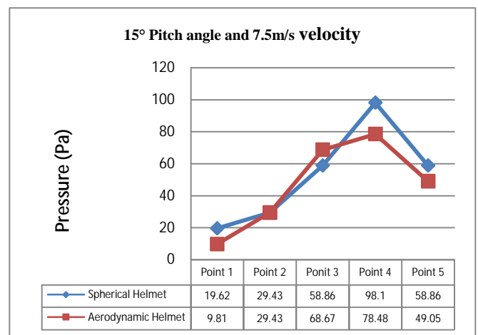
Graph5. At 15°Pitch angle and 7.5m/s velocity
