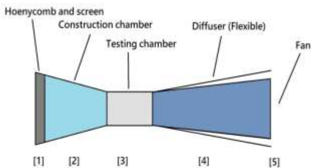
Figure 3. Wind Tunnel Diagram
