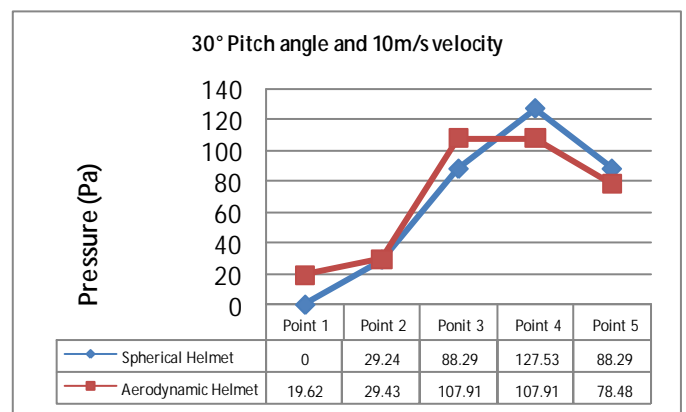
Graph9. At 30°Pitch angle and 10m/s velocity
