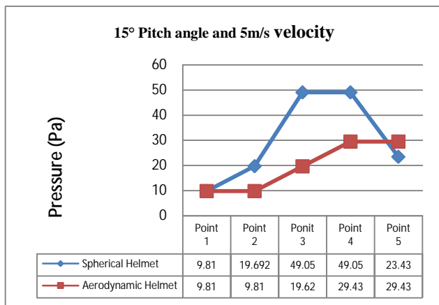
Graph2. At 15°Pitch angle and 5m/s velocity
