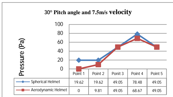
Graph6. At 30°Pitch angle and 7.5m/s velocity
