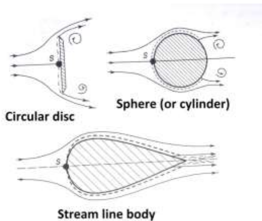
Figure 2. Wake-formation
