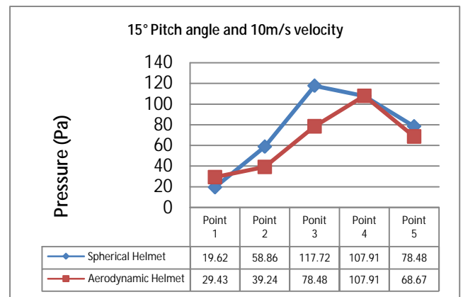
Graph8. At 15°Pitch angle and 10m/s velocity
