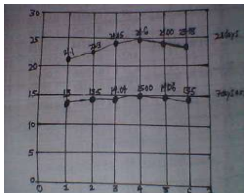
Compressive Strength Graph Variation in m20 after 7&28 days
