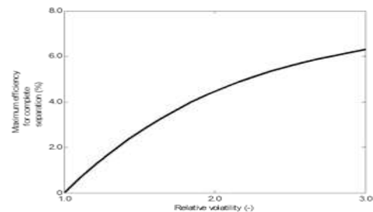
Figure 1. Effect of relative volatility on maximum efficiency for complete separation of a binary mixture by simple distillation
