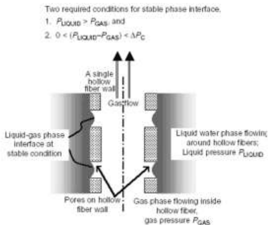
Figure 6. Liquid-gas interface in a membrane contactor
