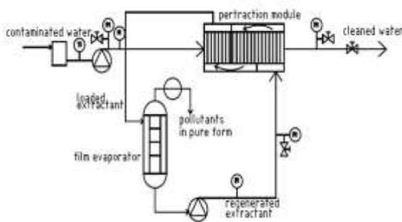
Figure 4. Scheme of a pertraction-regeneration process, with component released in pure form
