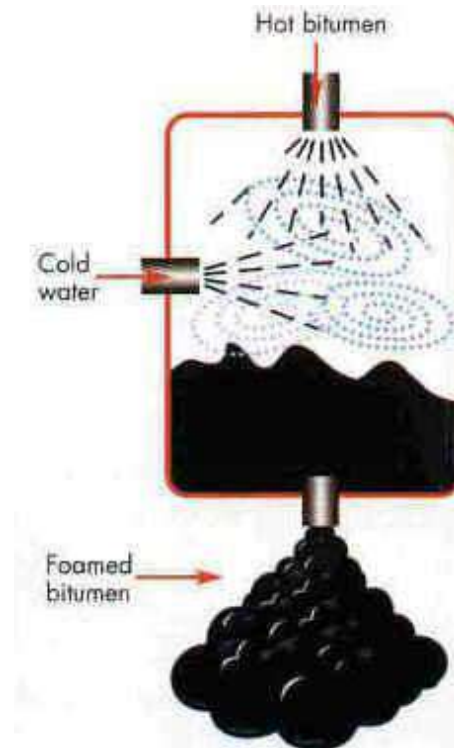
Figure 1 foaming of bitumen
