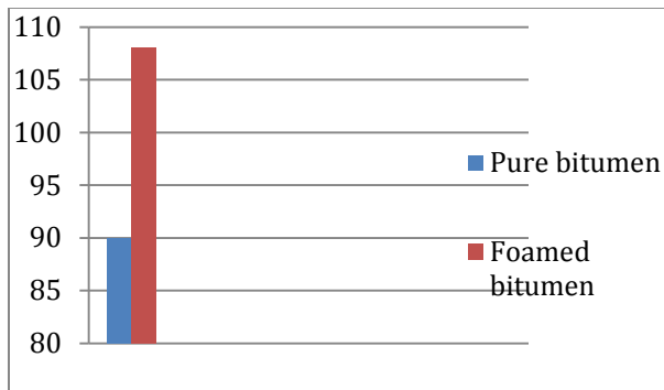
Figure 5 ductility graph
