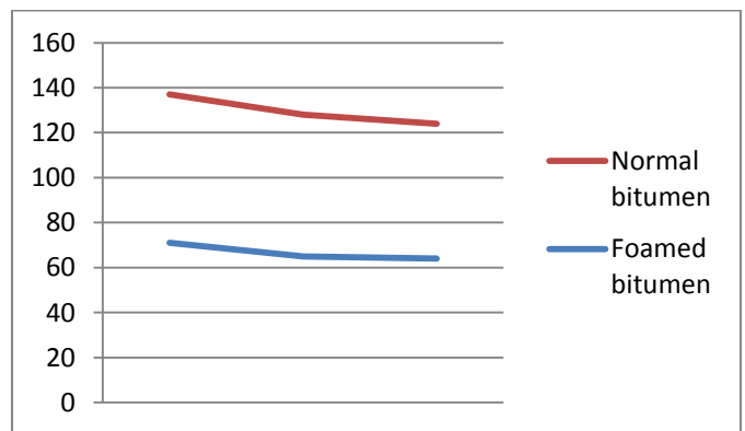
Figure 4 penetration graph
