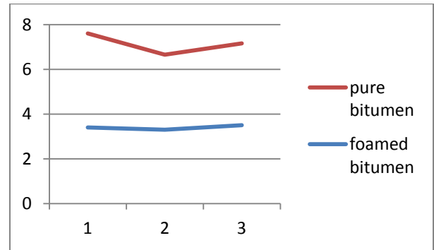
Figure 9 flow curve
