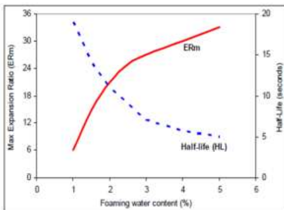
Figure 3 half life and expansion ratio
