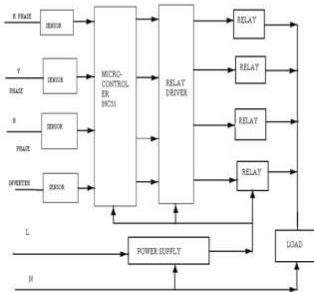
3.1 Block Diagram of Automatic Phase Changer
