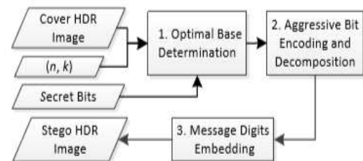
Fig. 2. Flowchart of embedding k secret bits into a pixel group of n pixels in the proposed DHOB algorithm.
