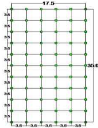
Figure 1. Plan of the building
