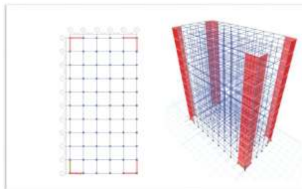
Figure 3. Model with corner Shear wall
