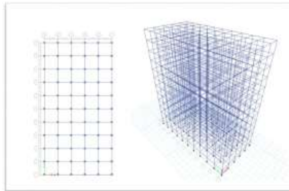
Figure 2. Model without Shear wall
