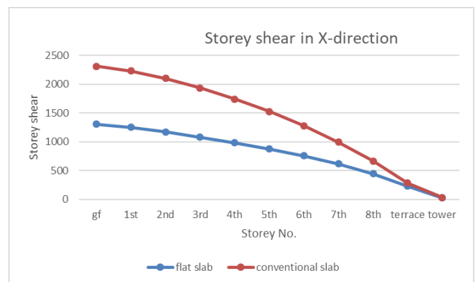
Chart -1: Storey shear in X-direction
