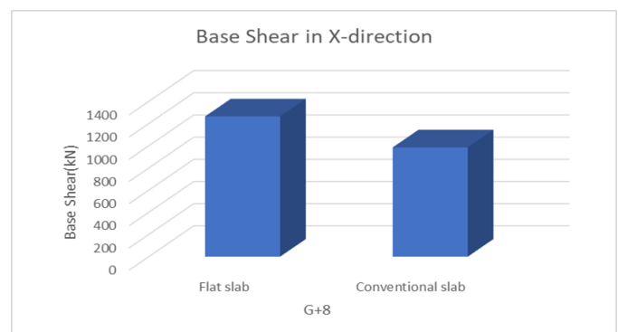
Chart -1: Base shear in X-direction
