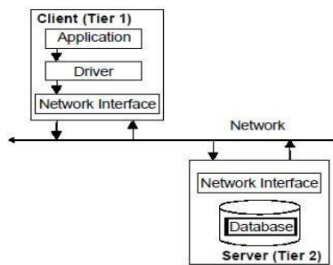
Figure 1: Two Tier Client/Server Architecture Model
