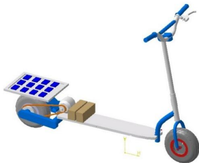
Fig - 5: Layout of hybrid bicycle
