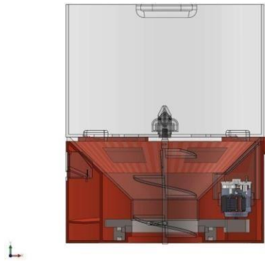
Fig.2.1 Storing Unit
