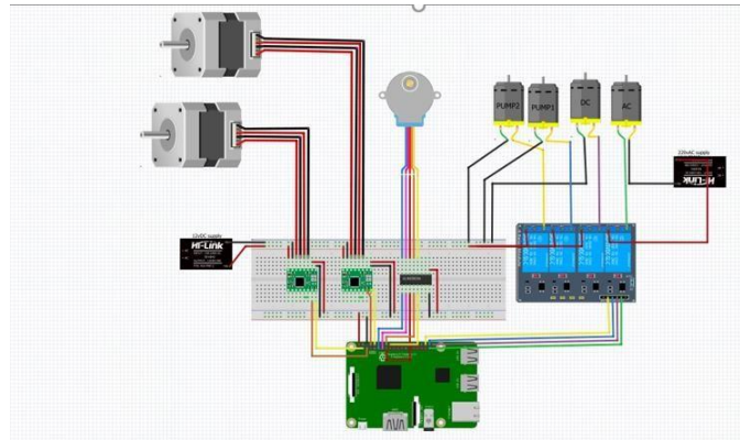
Fig 5.2 Circuit Diagram
