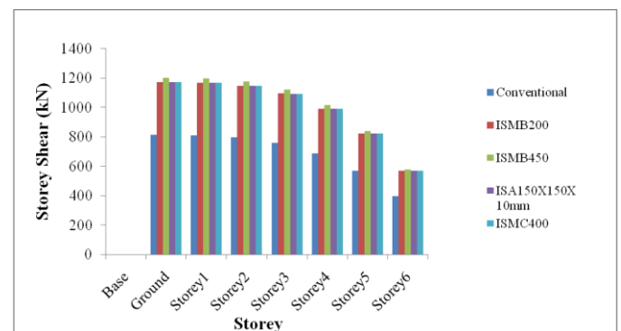
Chart -9: Storey shear along Y direction (EQy) in mm
