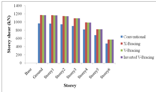
Chart -2: Storey shear along X (EQx) in kN
