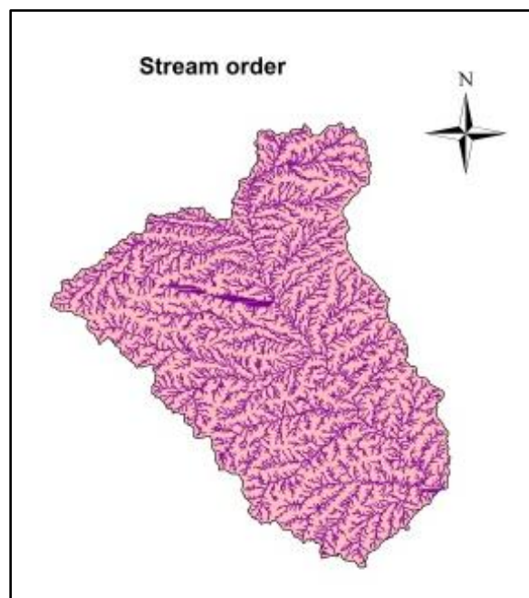
Figure 2. Stream Order of Sina Basin
